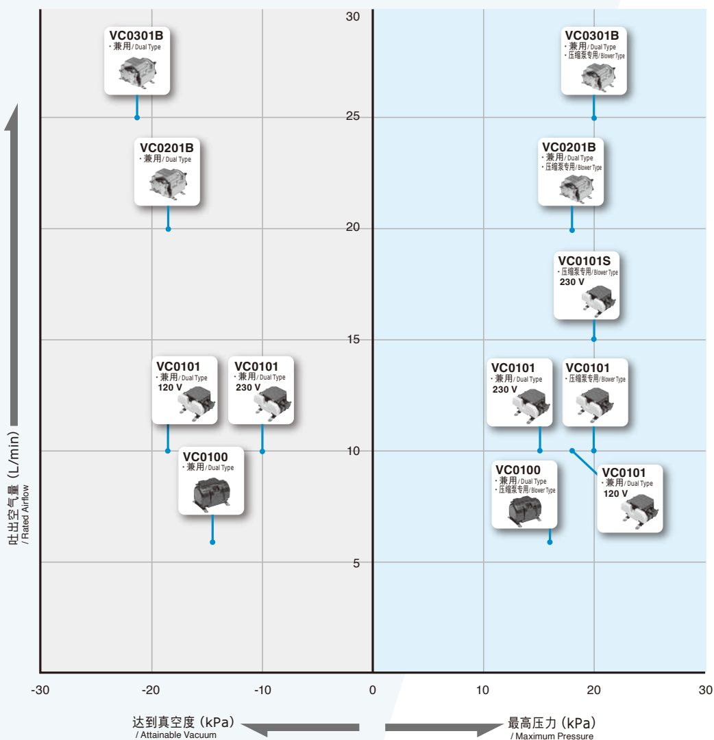
真空泵 / Vacuum Pump
