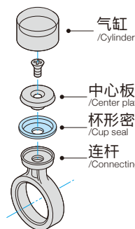
杯形密封系统 /Piston pump (Cup seal system)
